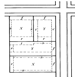
Transition Yards (t) Where X = residential lot, and Y = non-residential lot f = Front Yard c = Corner Side Yard s = Side Yard r = Rear Yard
