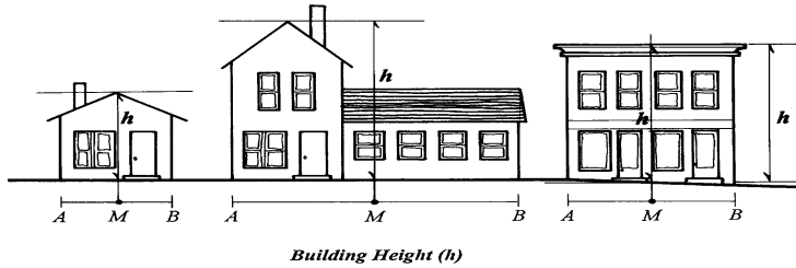
Where building height ( h ) is measured at M , the midpoint between A and B
